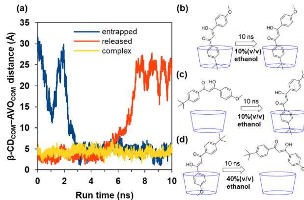
Fig. 6 (a) Plot of the \text{host}_{\text{COM}}-\text{AVO}_{\text{COM}} distance against the run time (ns) for three different AVO- \beta -CD systems: complex or (b) AVO- \beta -CD complex with a starting orientation of t -Bu inserted within the narrow rim in 10% ethanol, showing the typical behaviour of a host-guest complex with minimal fluctuation in the host-guest distance (remains complexed); entrapped or (c) AVO- \beta -CD complex with a starting orientation of AVO above \beta -CD in 10% ethanol, demonstrating guest entrapment; released or (d) AVO- \beta -CD complex with a starting orientation of MeO inserted within the narrow rim in 40% ethanol, demonstrating the departure of the guest from the host. These data demonstrate that sterics can contribute to the continual entrapment of AVO, regardless of the host, but favourable interactions and a lower ethanol content can also lead to entrapment. Note that water and ethanol molecules were omitted for clarity.
