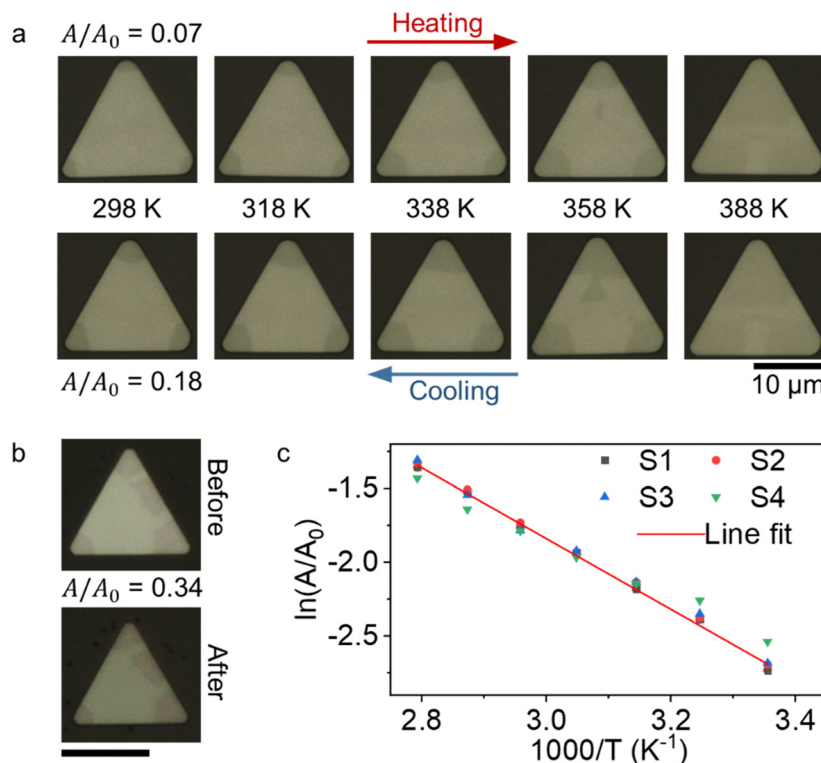
Fig. 3 (a) Optical microscopy micrographs of a \text{Cu}_2\text{Se} crystal taken during thermal cycling. After cooling down to room temperature, the A/A_0 ratio increases more than two times. (b) When thermal cycling is performed under 10^{-2} mbar vacuum, no change is measurable in A/A_0 . The scale bar is 10\ \mu\text{m} . (c) Arrhenius plot of A/A_0 versus T^{-1} for four different samples of similar size. The average activation energy is calculated from the slope of the lines fit to be E_A = 0.207 \pm 0.053\ \text{eV} .
