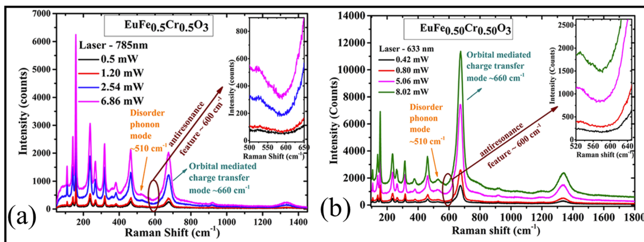
Fig. 4 Raman spectra for Cr-doped EuFe_{0.5}Cr_{0.5}O_3 samples using excitation wavelengths (a) 785 nm and (b) 633 nm at different laser powers. Reproduced from ref. 49 with permission from [American Chemical Society], copyright [2022].
