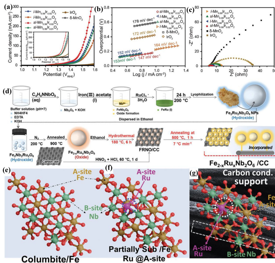
Fig. 5 (a) LSV curves (inset plot depicts LSV curves normalized by ECSA), (b) corresponding Tafel slopes, and (c) Nyquist plots of \text{Ir-Mn}_{0.98}\text{Ir}_{0.02}\text{O}_2 and its counterparts in 0.5 M \text{H}_2\text{SO}_4 (reproduced with permission from ref. 1. Copyright 2023, Wiley-VCH GmbH). (d) Schematic diagram depicting the synthesis process for \text{Fe}_{2-x}\text{Ru}_x\text{Nb}_2\text{O}_6/\text{carbon cloth} . Chemical structures of (e) \text{FeNb}_2\text{O}_6 , (f) \text{Fe}_{2-x}\text{Ru}_x\text{Nb}_2\text{O}_6 , and (g) \text{Fe}_{2-x}\text{Ru}_x\text{Nb}_2\text{O}_6/\text{carbon cloth} depicting the site occupancies in columbite (reproduced with permission from ref. 26. Copyright 2023, Wiley-VCH GmbH).
