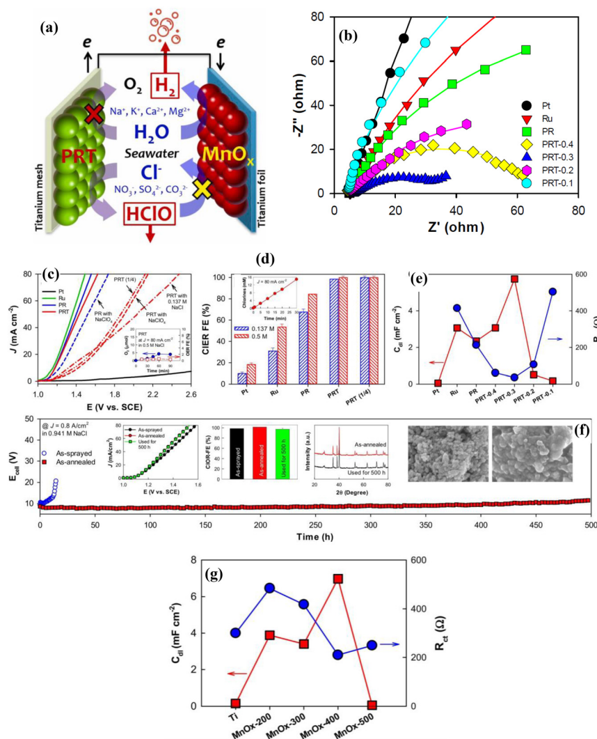
Fig. 7 (a) Schematic diagram illustrating seawater electrolysis using the MnO x cathode and PtRuTiO x (PRT) anode without using a membrane in a single compartment cell, where the CIER selective anode and HER selective cathode could eliminate the CIRR, while pure H 2 gas could be formed, where the chlorine generated could be in the aqueous form. (b) Nyquist plot of Pt 0.06 Ru 0.24 Ti 0.7 O y in comparison with those of its counterparts for CIER in simulated seawater electrolyte. (c) LSV curves for CIER of PRT in comparison with those of its counterparts in 0.5 M NaCl (pH 6), 0.137 M NaCl and 0.5 M NaClO 4 (pH 6), where PRT (1/4) indicates a mass loading of 0.83 mg cm -2 , while the inset depicts the CIER and faradaic efficiency (FE) of PRT at 80 mA cm -2 in 0.5 M NaCl. (d) FE of PRT in comparison with those of its counterparts for CIER at 80 mA cm -2 , where the inset depicts the production of free chlorine over time at 80 mA cm -2 . (e) R_{\text{ct}} and C_{\text{dl}} values obtained from the Nyquist plot of Pt 0.06 Ru 0.24 Ti 0.7 O y in comparison with those of its counterparts in simulated seawater electrolyte. (f) Long-term stability test for CIER of as-annealed PRT in comparison with that of as-sprayed PRT at 80 mA cm -2 in 0.941 M NaCl, where the inset depicts the LSV curves and FE for CIER of the as-sprayed and as-annealed materials and PRT used for 500 h at 80 mA cm -2 in 0.5 M NaCl, while the inset further shows the XRD patterns of the as-annealed material and PRT used for 500 h, and the inset further depicts the SEM images of the as-annealed material (left) and PRT used for 500 h (right). (g) R_{\text{ct}} and C_{\text{dl}} values obtained from the Nyquist plot of MnO x -400 in comparison with those of its counterparts for the HER in simulated seawater electrolyte (reproduced with permission from ref. 25. Copyright 2022, Elsevier B.V.).
