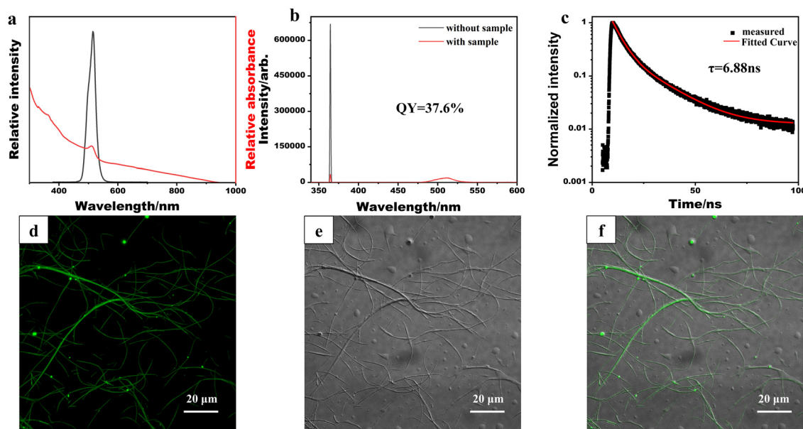
Fig. 3 Optical characterization of CsPbBr 3 /PbSe nanowires: (a) UV/vis absorption and photoluminescence spectra, (b) PLQY, (c) lifetime, (d) confocal fluorescence image, (e) bright field image and (f) merged image of (d) and (e).
