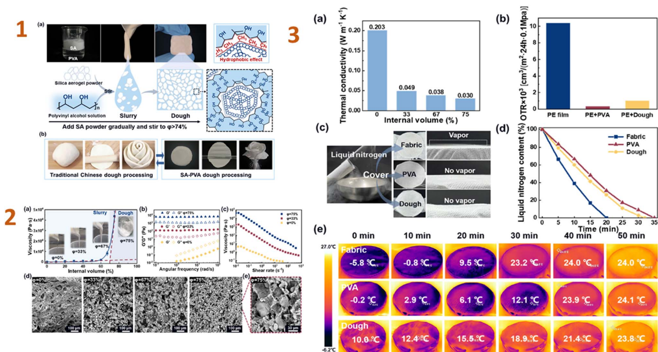
Fig. 11 (1) Formation of the SA–PVA dough. (a) Schematic diagram of the formation of high internal phase structure in the SA–PVA dough. (b) Similar moulding properties of the SA–PVA dough to traditional Chinese dough; (2) (a) changes in viscosity during the formation of the dough. (b) Changes in G' (storage modulus) and G'' (loss modulus), (c) variation of viscosity with shear rate and (d and e) SEM images of the composites with different SA contents; (3) (a) thermal conductivity of as-prepared PVA/SA composite materials with different SA content. (b) A comparison of oxygen permeation rates for PE film, PVA coating, and dough coating. (c) Experimental design for thermal insulation and gas barrier properties of the dough. (d) Changes in liquid nitrogen weight over time under the encapsulation and (e) surface temperature changes over time using FLIR testing under the encapsulation of PE film, PVA coating, and dough coating. This figure has been adapted/reproduced from ref. 146 with permission from Elsevier under the license number 5823680861420, copyright 2024.
