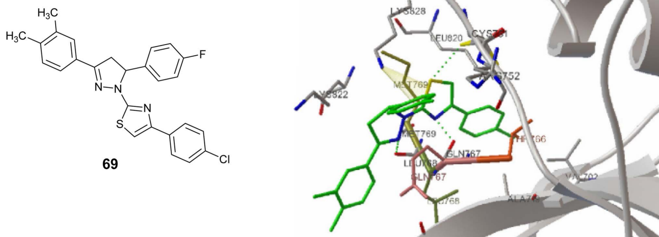
Fig. 32 Molecular docking modeling of compound 69 with EGFR Masse.
