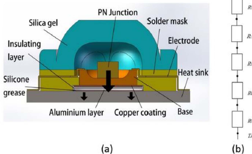
Fig. 11 (a) LED cooling system and (b) its corresponding thermal resistance network. Reproduced with permission 138 copyright © 2022 Springer Nature.
