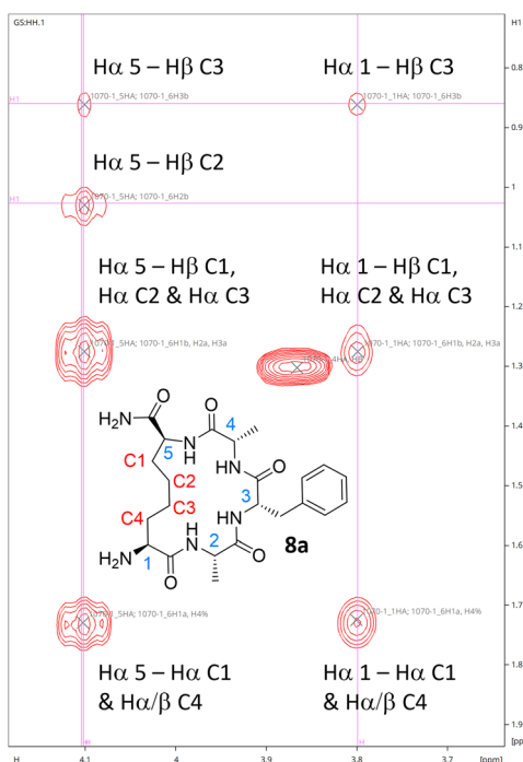
Fig. 3 Ha region for the TOCSY NMR spectrum of 8a confirming successful formation of the macrocycle.
