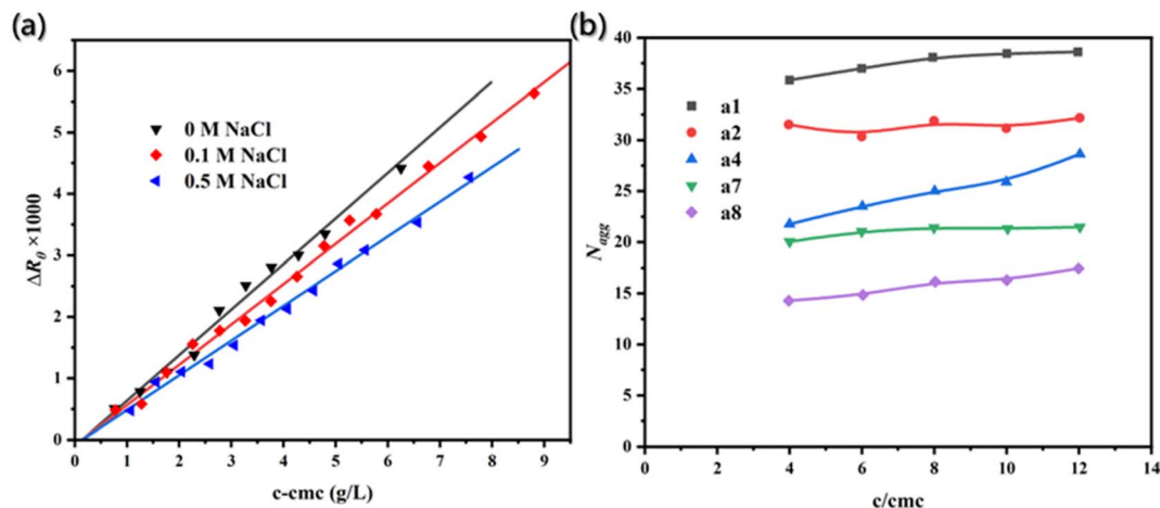
Fig. 4 (a) Excess scattering ratios ( \Delta R_{\theta} ) is the function of micellar concentration. 89 Reproduced with permission from ref. 89. Copyright 2007, Elsevier. (b) Aggregation number ( N_{agg} ) as a function of concentration c/cmC with different carbon atomic number ( s ) spacing between two dodecyl chains and a diamide spacer. 90 Reproduced with permission from ref. 90. Copyright 1999, American Chemical Society.
