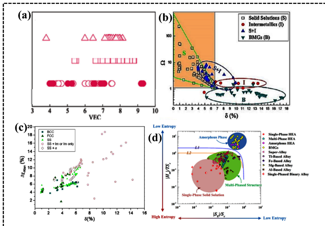
Fig. 6 (a) Effect of valence electron concentration (VEC) on phase stability in HEAs. The symbol \circ represents equiatomic amorphous phase forming alloys; \bullet represents non-equiatomically amorphous phase forming alloys; \square represents solid solution phases and \triangle represents intermetallic phases. Reproduced with permission. 78 Copyright 2011, Elsevier Ltd. (b) Relationship between parameters. Reproduced with permission. 88 Copyright 2012, Elsevier Ltd. (c) Radius versus electronegativity mismatch for HEAs. Reproduced with permission. 82 Copyright 2014, Elsevier Ltd. (d) Thermodynamic phase diagram of HEAs. Reproduced with permission. 89 Copyright 2015, Elsevier Ltd.
