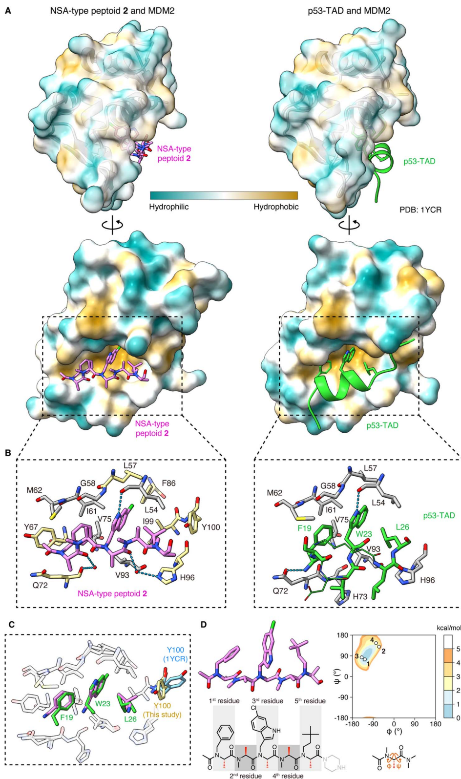
Fig. 2 Crystal structure of peptoid 2 bound to MDM2 (A) crystal structure of 2 (pink, left) and p53-TAD (light green, right) (PDB ID 1YCR) bound to MDM2. The surface color of MDM2 represents the hydrophobicity. (B) A close-up view of the interface between (left) 2 (pink) and MDM2 (gray and yellow) or (right) p53-TAD (light green) and MDM2 (gray). Only the MDM2 residues that make van der Waals contacts with 2 or Phe19–Leu26 of p53-TAD are shown. In the left figure, the MDM2 residues also shown in the right figure are colored gray and the unique ones in the left are colored yellow. The hydrogen bond is shown as a cyan dashed line. (C) Overlay of the crystal structure of 2 (pink) complexed with MDM2 (white) and p53-TAD (light green) complexed with MDM2 (white) (PDB ID 1YCR), aligned by MDM2. Only MDM2 residues in van der Waals contact with 2 or Phe19–Leu26 of p53-TAD are shown. The Tyr100 residue of MDM2, which is in different orientations in the two structures, is also shown
