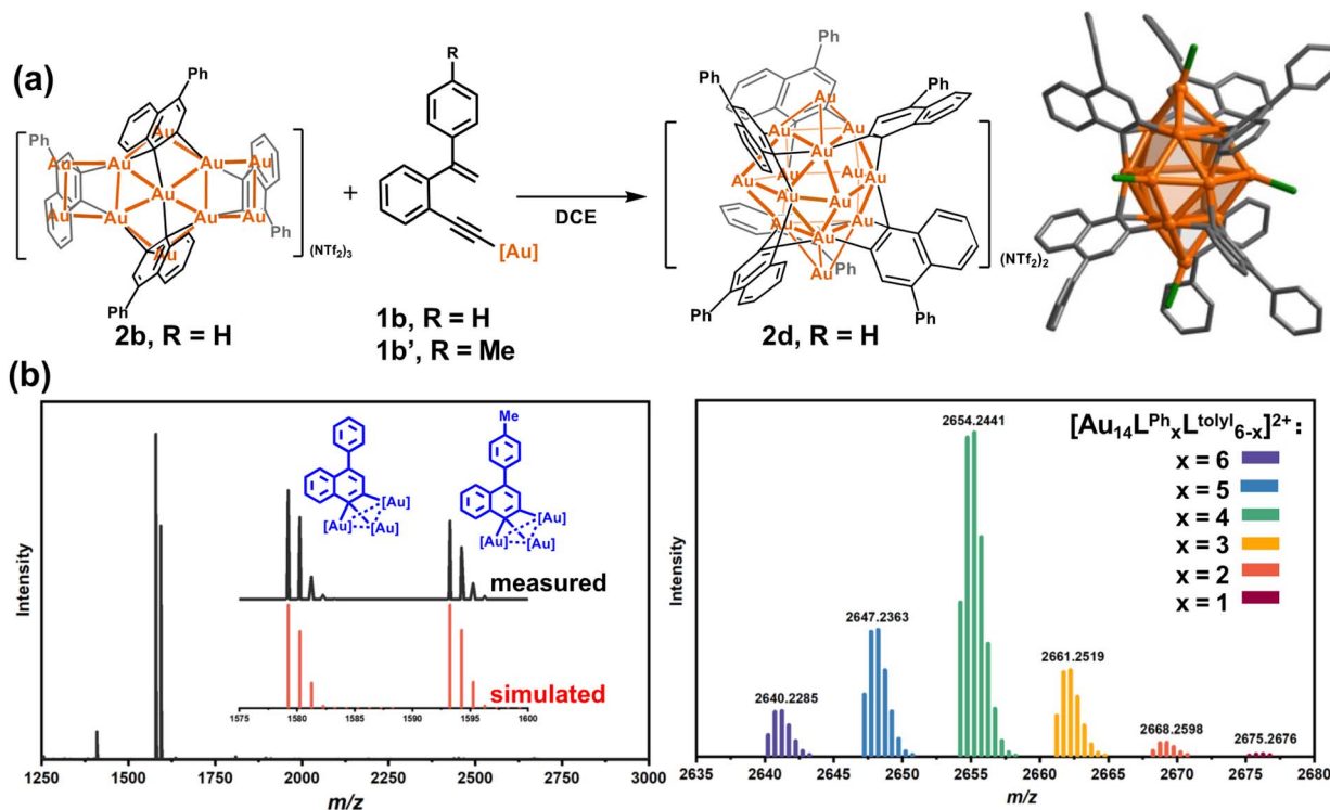
Fig. 2 (a) The 2b-to-2d transformation and crystal structure of 2d. Phenyl groups of \text{PPh}_3 ligands, hydrogen atoms, and peripheral \text{NTf}_2^- counter anions are omitted for clarity. Color coding: Au, yellow; C, gray; P, green. (b) (Left) The in situ ESI mass spectra of the crossover experiment between 2b and 1b', and (right) ESI-MS of deposited microcrystals.
