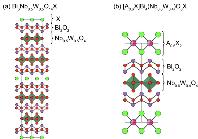
Fig. 16 Crystal structures of (a) \text{Bi}_6\text{Nb}_{0.5}\text{W}_{0.5}\text{O}_{14}\text{X}^{133} and (b) [\text{A}_{0.6}\text{X}]\text{Bi}_4(\text{Nb}_{0.6}\text{W}_{0.4})\text{O}_8\text{X} ( \text{A} = \text{K}, \text{Rb}, \text{Cs} ). 134 Note that non-distorted ideal structures are shown for clarity.
