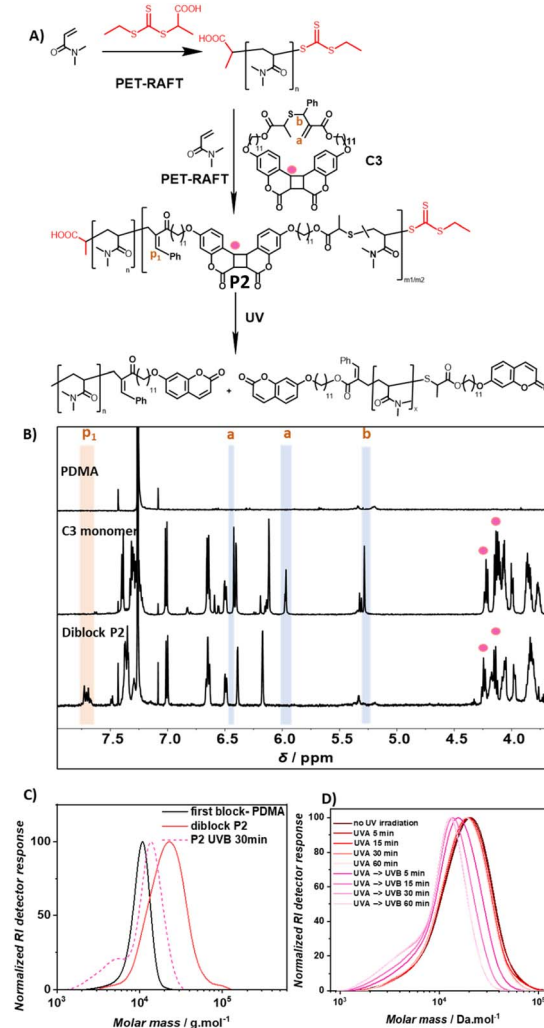
Fig. 3 (A) Synthesis of diblock copolymer P2 , PDMA- b -(DMA-co- C3 ), of coumarin based monomer C3 and DMA, and its photodegradation under UV light. Protons whose resonances change in the ^1\text{H} NMR are denoted with orange letters; (B) ^1\text{H} NMR spectra of PDMA, cyclic monomer C3 and copolymer P2 (PDMA- b -(DMA-co- C3 )); (C) overlaid SEC traces of the first PDMA block, diblock copolymer P2 and UVB degraded P2 in DMAc; (D) SEC traces of polymer P2 in DMAc solution over the course of UVA and UVB irradiation.
