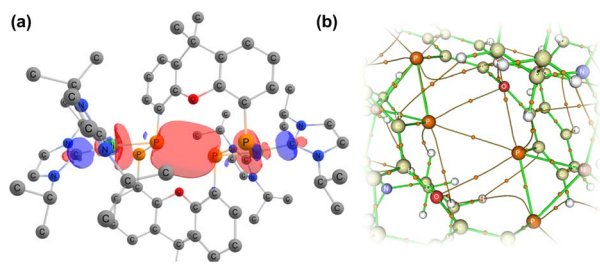
Fig. 5 (a) Combination of orbitals leading to a cross-ring P–P interaction, found through a second-order perturbation theory analysis of 2 ; (b) a QTAIMs analysis of 2 indicating a bond critical point between P1 and P1'.
