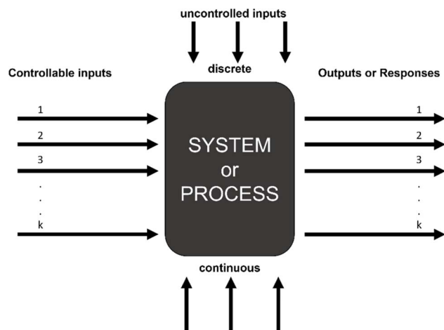
Fig. 1 Black box representation of DOE. 16
