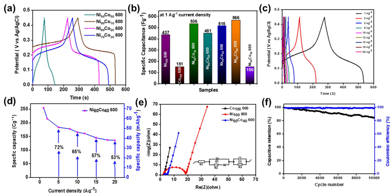
Fig. 6 (a) GCD curves (recorded within 0–0.45 V and 1 A g -1 ), (b) bar diagram showing the C_{sp} for the as-prepared material with different Ni/Co ratios, (c) GCD curves of activated Ni 60 Co 40 600 at various current densities (1–20 A g -1 ), (d) C_s vs. current density plot, (e) Nyquist plot for activated Ni 100 600, Co 100 600 and Ni 60 Co 40 600 (inset shows the Randles circuit for impedance data fitting, where R , W , C , and Q parameters are the resistor, Warburg impedance, capacitor, constant phase element, respectively), and (f) durability test of activated Ni 60 Co 40 600, performed at constant 10 A g -1 current density (up to 10 000 cycles).
