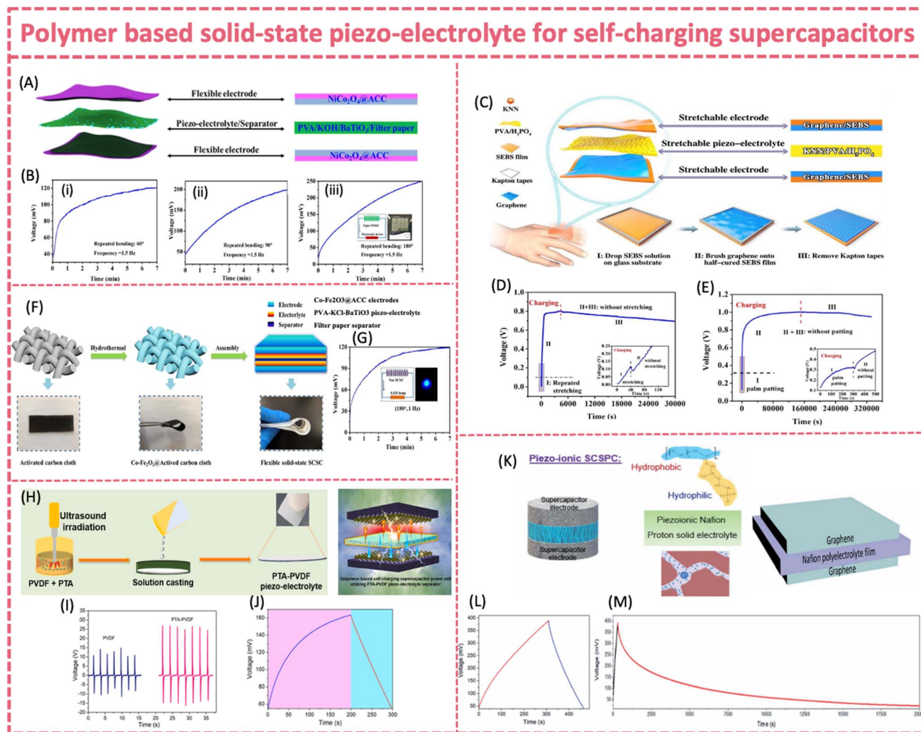
Fig. 13 (A) Structure of an FSSSC made of two \text{NiCo}_2\text{O}_4@\text{ACC} electrodes, a PVA/KOH/BaTiO 3 piezoelectrolyte, and a filter paper separator. (B) Self-charging behavior at (i) 60°, (ii) 90°, and (iii) 180° repeated bending. Reproduced from ref. 142 with permission from American Chemical Society, copyright 2020. (C) Structure of a stretchable SCSC consisting of graphene/SEBS electrodes and KNN/PVA/H 3 PO 4 piezo-electrolyte. (D) Self-charging process of a single device under repeated stretching for about 40 s. (E) Four serially connected devices under palm patting for 300 s. Reproduced from ref. 140 with permission from the Royal Society of Chemistry, copyright 2020. (F) Synthesis and corresponding photographs of the Co-Fe 2 O 3 @ACC electrode and architecture of the flexible solid-state SCSC. (G) Self-charging curves at 180° repeated bending. Reproduced from ref. 141 with permission from Elsevier, copyright 2021. (H) Preparation of PTA-PVDF piezo-polymer-electrolyte for use in SCSPCs. (I) Current and voltage outputs of the PTA-PVDF film. (J) Self-charging performance of a graphene SCSPC subjected to a compressive force of 2 N. Reproduced from ref. 143 with permission from Elsevier, copyright 2021. (K) Structure of a piezo-ionic SCSPC and molecular structure of Nafion and the ionomeric cavity present in Nafion. (L) Self-charging properties of graphene PI-SCSPC recorded at 10 m s -2 and (M) self-discharge profiles of graphene PI-SCSPC monitored over 20 000 seconds. Reproduced from ref. 55 with permission from the Royal Society of Chemistry, copyright 2022.
