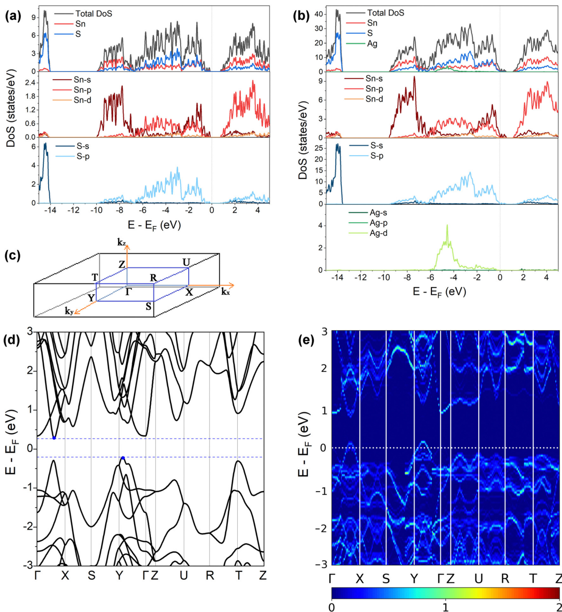
Fig. 3 (a) and (b) Total and atom-projected (partial) density of states of pristine SnS (a) and 2.78% Ag-doped SnS (b) calculated at the HSE06 level of theory. (c) Pmcn Brillouin zone with high-symmetry points marked. (d) and (e) Electronic band structures of pristine SnS (d) and 2.78% Ag-doped SnS (e) calculated at the PBEsol level of theory.
