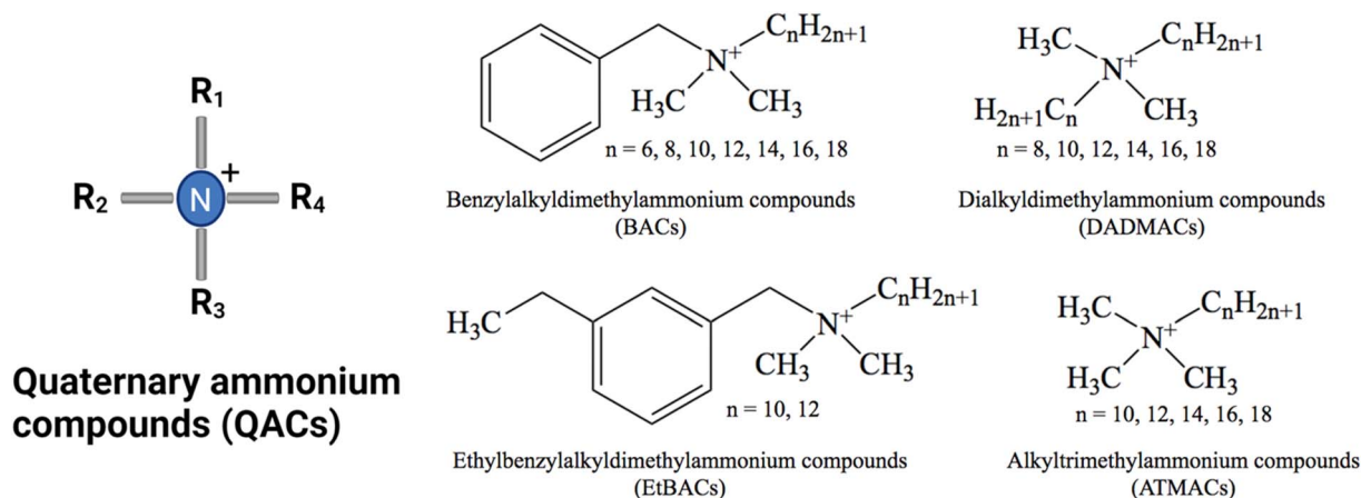
Fig. 1 General structure of the four main QAC chemical groups. The most commonly used QACs are C 8 –C 18 BAC, C 12 –C 14 EtBAC and C 8 , C 8/10 and C 10 DADMAC. 33
