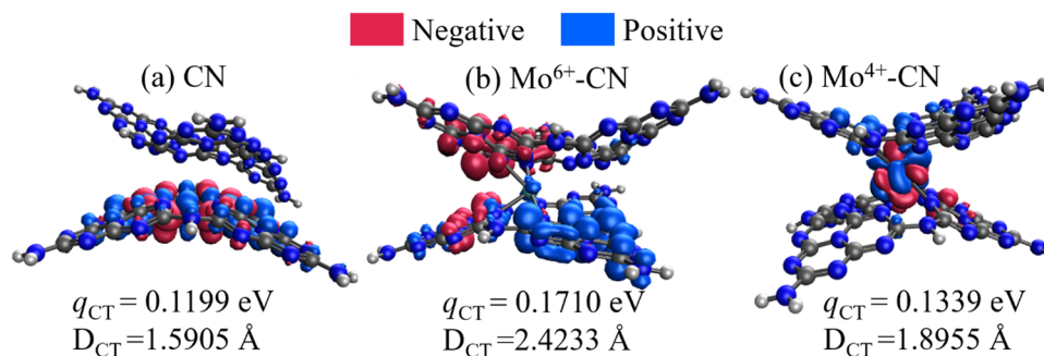
Fig. 9 First excited state of the electron/hole distribution of CN (a), Mo^{6+} -CN (b), and Mo^{4+} -CN (c). The intramolecular electron transition distance ( D_{CT} ) and the intramolecular charge transfer amount ( q_{CT} ) are given.
