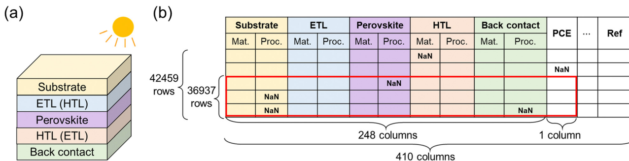
Fig. 1 The structures of perovskite solar cell and the Perovskite Database. (a) Typical structure of n-p-type cell, and the bracket represents the pin-type structure. (b) The size and information of the Perovskite Database. The curated dataset used in this work is shown by red boxed line.
