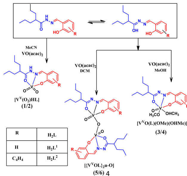
Scheme 1 Schematic of the synthesis of the complexes.
