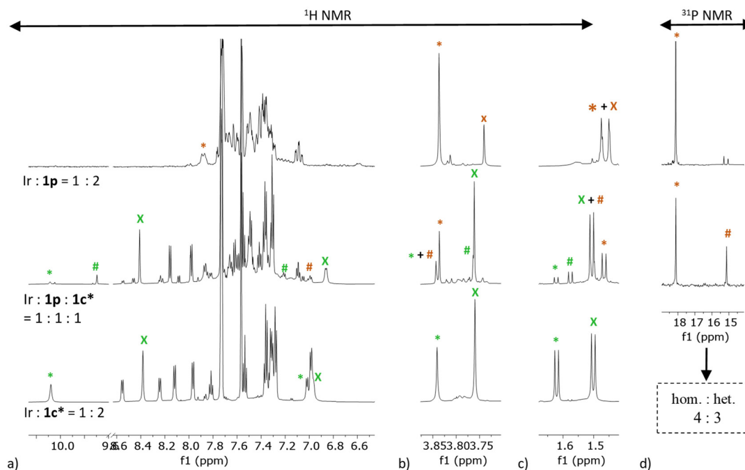
Fig. 5 Stacked ^1\text{H} NMR spectra (CD _2 Cl _2 ) of homoleptic and heteroleptic solutions of [Ir(COD) _2 ]BARf precursor and 1p ligand (orange) or/and 1c* ligand (green): (a) aromatic region, (b) functional group region, (c) aliphatic region. (d) Stacked ^{31}\text{P} NMR spectra. The homoleptic peaks are indicated by an asterisk (*), the heteroleptic peaks are indicated by a hash sign (#), the free ligand peaks are indicated by the letter (X). Abbreviations: hom.-homoleptic species; het.-heteroleptic species.
