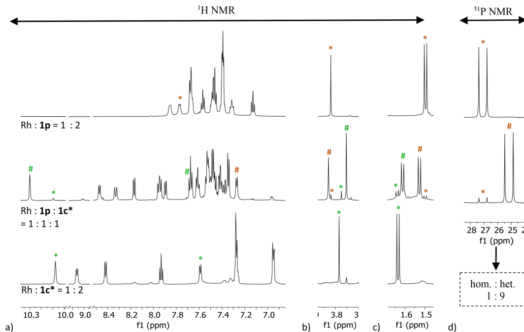
Fig. 4 Stacked ^1\text{H} NMR spectra (CD _2 Cl _2 ) of homoleptic and heteroleptic solutions of [Rh(COD) _2 ]BF _4 precursor and 1p ligand (orange) or/and 1c* ligand (green): (a) aromatic region, (b) functional group region, (c) aliphatic region. (d) Stacked ^{31}\text{P} NMR spectra. The homoleptic peaks are indicated by an asterisk (*) and the heteroleptic peaks are indicated by a hash sign (#). Abbreviations: hom.-homoleptic species; het.-heteroleptic species.
