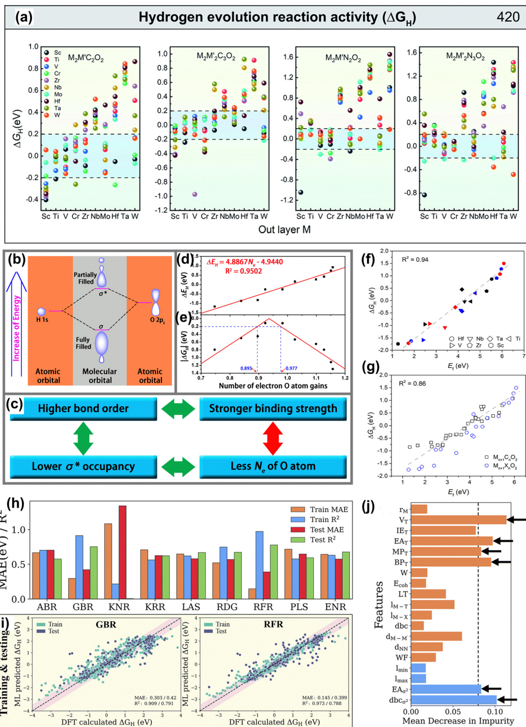
Fig. 12 (a) \Delta G_H distribution of hydrogen adsorbed by M_2M'X_2 and M_2M'X_3O_2 , and the black dotted line range represents |\Delta G_H| < 0.2 eV of MXene on equilibrium H coverage. 187 Reproduced with permission, ref. 187. Copyright 2020, Royal Society of Chemistry. (b) Schematic of the formation of the H–O bond on the surface of O-terminated MXene, where the linear combination of a H 1s orbital and an O 2p z orbital forms a fully filled, low-energy bonding orbital ( \sigma ) and a partially filled, high-energy antibonding orbital ( \sigma^* ). (c) The derivation of the correlation between the N_e of the O atom and the H–O binding strength. The calculated (d) \Delta E_H and (e) |\Delta G_H| as a function of the number of electron O atom gains ( N_e ), where the R^2 is 0.95, indicating the high linear correlation between the N_e and \Delta E_H . 188 Reproduced with permission, ref. 188. Copyright 2016, American Chemical Society. (f) Linear relationship between the oxygen vacancy formation energy ( E_f ) and free energy of hydrogen adsorption ( \Delta G_H ) of M_{n+1}N_nO_2 . The black, red, and blue symbols represent M_2XO_2 , M_3X_2O_2 and M_4X_3O_2 , respectively. (g) The linear relationship between E_f and \Delta G_H of both M_{n+1}C_nO_2 and M_{n+1}N_nO_2 . The gray dashed line represents linear fitting of the data. 189 Reproduced with permission, ref. 189. Copyright 2018, American Chemical Society. (h) Mean absolute error (MAE) and coefficient of determination ( R^2 score) of the ABR, ENR, GBR, KNR, KRR, LAS, PLS, RFR and RDG algorithms using primary (atomistic, structural and electronic indicators) and statistical function-processed features. (i) Parity plots of the best-performing RFR and GBR models using the DFT dataset of hydrogen adsorption Gibbs free energies ( \Delta G_H ). The pink-shaded regions indicate a deviation of up to 0.5 eV. (j) Feature importance from the mean decrease in impurity for the GBR model with RFE-HO-LOO, evaluated via 20-fold cross-validation. 178 Reproduced with permission, ref. 178. Copyright 2023, Royal Society of Chemistry.
