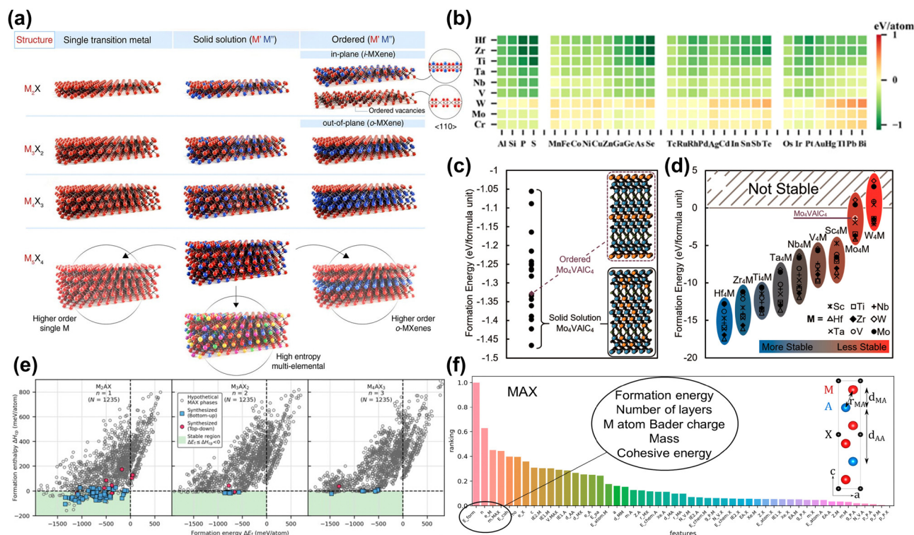
Fig. 2 (a) Schematic illustration of the MXene structures. 24 Reproduced with permission ref. 24. Copyright 2021, AAAS. (b) \Delta E_f for 288 \text{M}_2\text{AC} phases displayed as a heatmap for 9 metals and 32 different elements at the A site. 69 Reproduced with permission ref. 69. Copyright 2023, Elsevier. (c) Formation energies for solid-solution \text{Mo}_4\text{VAIC}_4 configurations (black dots) compared to ordered \text{Mo}_4\text{VAIC}_4 (purple diamond). (d) DFT calculated formation energies of ordered \text{M}'_4\text{M}''\text{AlC}_4 MAX phases. Most are predicted to be stable except for some Mo and W compositions. 70 Reproduced with permission ref. 70. Copyright 2019, American Chemical Society. (e) Calculated formation enthalpy \Delta H_{cp} as a function of formation energy \Delta E_f for ternary \text{M}_{n+1}\text{AX}_n phases with n = 1, 2, 3 . Hypothetical MAX phases are given by grey circles and synthesized MAX phases by blue squares (bottom-up synthesis) and red hexagons (top-down synthesis). The green area marks the region of thermodynamic stability fulfilling \Delta H_{cp} < 0 (and \Delta E_f < 0 ). 71 Reproduced with permission, ref. 71. Copyright 2024, Elsevier. (f) Feature importance ranking for MAX. Layer distances and bond lengths are labeled in the unit cell diagrams. 72 Reproduced with permission, ref. 72. Copyright 2017, American Chemical Society.
