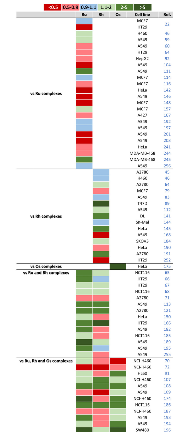
Fig. 30 A comparison of the relative activity (RA) of Ir complexes with their Ru, Rh and/or Os analogues. RA = IC 50 (Ru/Rh/Os complex)/IC 50 (Ir complex). The best-performing Ir complexes and the data from lung cancer cells (where possible) were chosen for these comparisons.
