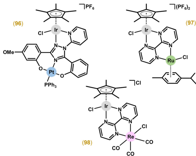
Fig. 24 Structural formulas of heterometallic complexes 96–98.
