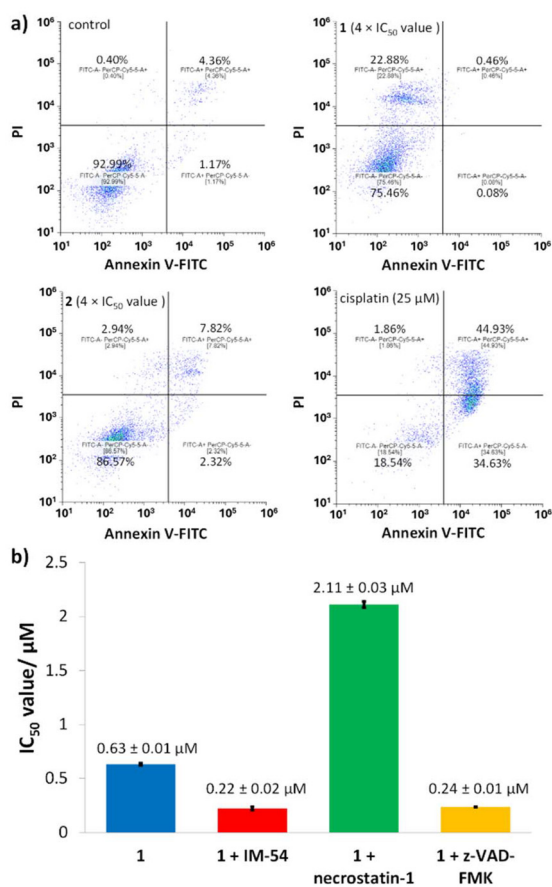
Fig. 6 (a) FITC Annexin V-propidium iodide binding assay plots of untreated HMLER-shEcad cells and HMLER-shEcad cells treated with 1 ( 4 \times IC_{50} value for 72 h) or 2 ( 4 \times IC_{50} value for 72 h) or cisplatin (25 \mu M for 72 h). (b) Graphical representation of the IC_{50} values of 1 towards HMLER-shEcad cells in the absence and presence of IM-54 (10 \mu M), necrostatin-1 (20 \mu M) or z-VAD-FMK (5 \mu M). Error bars represent standard deviations.
