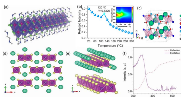
Fig. 4 (a) Views of a 1D Sn bromide wire wrapped by organic cations. 64 Copyright 2017 Wiley-VCH. (b) The variation in the integrated emission intensity ( \lambda_{\text{ex}} = 416 nm) of \text{CsMnCl}_3(\text{H}_2\text{O})_2 vs. the heating temperature (20–300 °C). Inset in the upper right shows the temperature-dependent PL spectra of \text{CsMnCl}_3(\text{H}_2\text{O})_2 . 65 Copyright 2020 Wiley-VCH. (c) Crystal structure of \text{CsMnCl}_3(\text{H}_2\text{O})_2 , hydrogen bonds (O–H) depicted as black dashed lines. 65 Copyright 2020 Wiley-VCH. (d) Structure of 1D \text{CsCu}_2\text{I}_3 SC (green: Cs atom, yellow: I atom, dark blue: Cu atom, purple octahedron: Cu–I octahedron). 66 Copyright 2019 Wiley-VCH. (e) Cu–I 1D chain surrounded by Cs atoms and the independent Cu–I chain that is like a “nanowire”. 66 Copyright 2019 Wiley-VCH. (f) Ultraviolet excitation spectrum collected at 568 nm and reflection spectrum. 66 Copyright 2019 Wiley-VCH.
