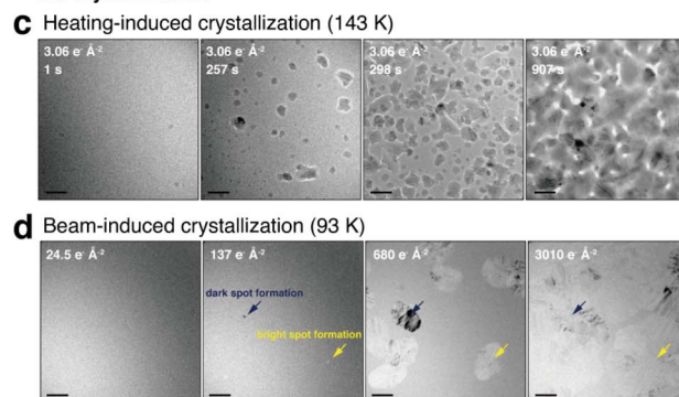
Fig. 8 Investigation and benchmarking of electron-beam effects on different samples. (a) Li dendrite image before high-resolution imaging attempt using conventional, room temperature TEM. (b) Li dendrite after beam damage caused by high electron doses after attempting high-resolution (reproduced with permission from ref. 26, copyright 2017 AAAS). (c) Example of heating-induced crystallization of ice, which is the intended process to be observed. (d) Example of beam-induced crystallization of ice from continuous irradiation, which produces artifacts that are different from the crystallization process observed by heating (reproduced with permission from ref. 136, copyright 2023 Nature Publishing Group). (e–l) Aligned and summed images of the protein hemoglobin embedded in vitreous ice, in which (a and e) are low-flux, (b and f) are medium-flux, (c and g) are high-flux, and (d and h) are high-flux short-exposure. (a–d) are 50 e Å -2 and (e–h) are 250 e Å -2 . (m) Plots of FRPR and FRC according to different dose rates calculated in MGy, providing information on the changes in low-resolution information according to accumulated dose. The threshold value of 45 deg for FRPR and 0.5 for FRC can be used to benchmark imaging dose rates (reproduced with permission from ref. 178, copyright 2011 IUCr Journals).
