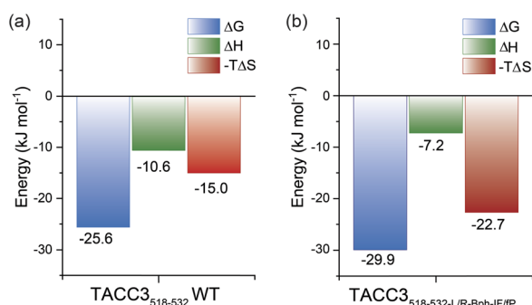
Fig. 5 Thermodynamics of binding in the presence of Aurora-A: (a) ITC thermodynamic signatures of linear TACC3 518-532 ; (b) constrained TACC3 518-532-L/R-Bph-IF/FP binding to Aurora-A 122-403-C290A/C393A . Data is shown as the average \pm SD of two independent titrations of the protein (46 \mu M) in 25 mM Tris buffer, 150 mM NaCl, 5 mM MgCl 2 , 5% v/v glycerol at pH 7.5.
