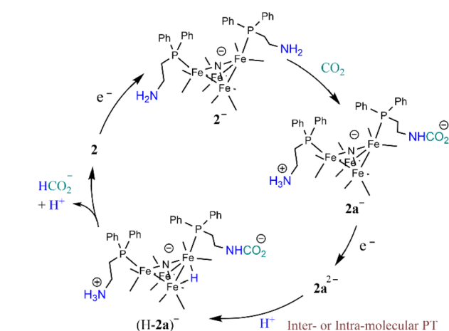
Scheme 3 Proposed mechanism for \text{CO}_2 reduction to formate by 2^- .
