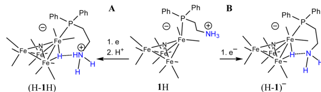
Scheme 2 Presentation of possible H-bond stabilization that enables observation of (\text{H-1H})^{0/-} or (\text{H-1a})^{2-} , couple at -1.63 V. (A) Proton source is from bulk solution; (B) proton source for hydride formation is the amine SCS group.
