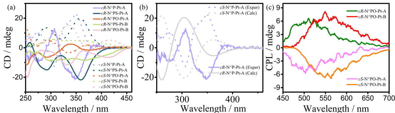
Fig. 9 (a) CD spectra of Pt(II) complexes in dilute CH 2 Cl 2 solution ( 3.0 \times 10^{-5} mol dm -3 ); (b) experimental and calculated CD spectra of cR/cS-N P -Pt-A complexes in dilute CH 2 Cl 2 solution; (c) CPL spectra of Pt(II) complexes in powder.
