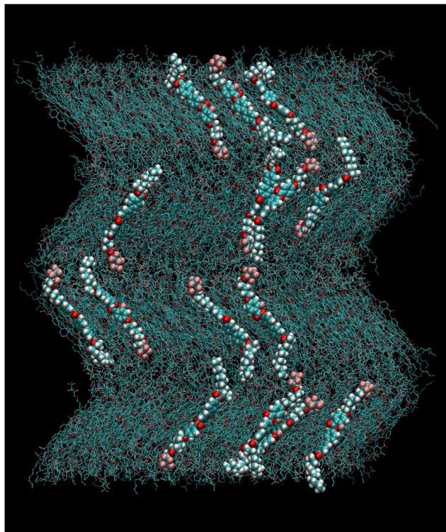
Fig. 5 Snapshot of the box with molecules in the orthoconic phase used for the NVT production run at T = 400 K. A few selected molecules are highlighted for clarity.
