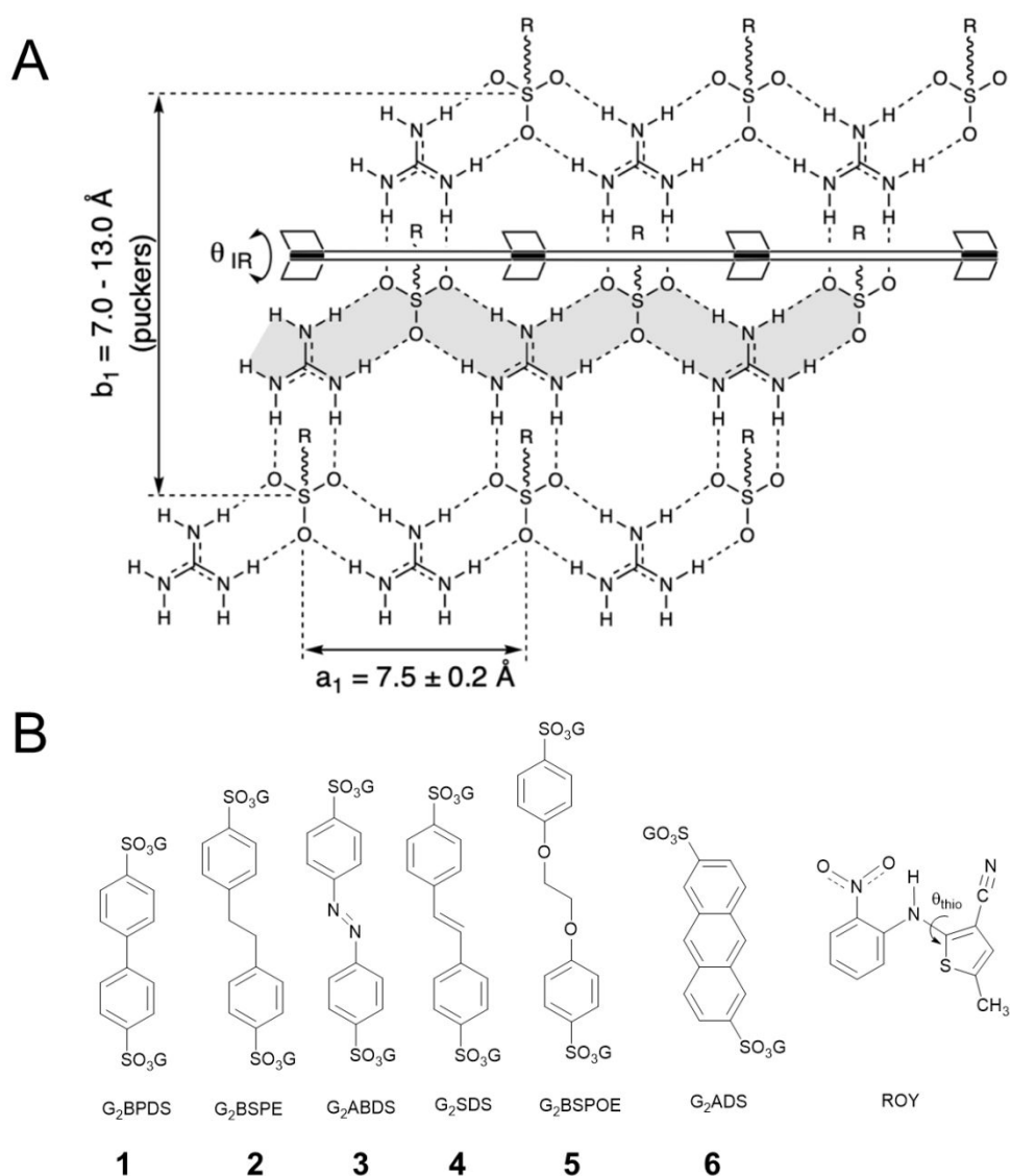
Fig. 1. (A) The quasi-hexagonal GS hydrogen bonded sheet illustrating the hydrogen-bonded major ribbons (one of these is highlighted in grey). (B) Molecular structures of the components in the guanidinium organosulfonate frameworks used herein and the molecular structure of ROY. The S-C-N-C torsion angle is denoted as \theta_{\text{thio}} . The numbers beneath the organosulfonate pillars correspond to their respective ROY inclusion compounds.
