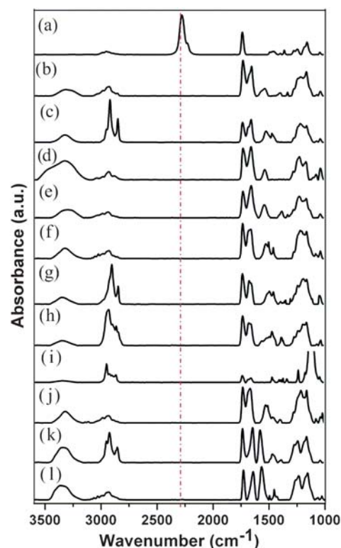
Fig. 3 GATR-FTIR spectra of brushes on \text{SiO}_x substrates (key peaks are identified): (a) poly(2-isocyanatoethyl methacrylate) brush ( 2275\text{ cm}^{-1} , NCO) (red) reacted with (b) 3-mercaptopropionic acid ( 3320\text{--}3000\text{ cm}^{-1} , COO–H), (c) 1-dodecanethiol ( 2954, 2924, 2852\text{ cm}^{-1} , C–H), (d) 1-thioglycerol ( 3573\text{--}3125\text{ cm}^{-1} , OH), (e) N -acetyl-L-cysteine ( 3450\text{--}3162\text{ cm}^{-1} , CO–NH), (f) benzyl mercaptan ( 3084, 3058, 3025\text{ cm}^{-1} , =C–H; 1517, 1493, 1451\text{ cm}^{-1} , C=C), (g) 1-adamantanethiol ( 2906, 2850\text{ cm}^{-1} , C–H), (h) thiocholesterol ( 2936, 2903, 2865, 2850\text{ cm}^{-1} , C–H), (i) 3-mercaptopropyl polyhedral oligomeric silsequioxane ( 1109\text{ cm}^{-1} , Si–O), (j) furfuryl mercaptan ( 1204, 1156\text{ cm}^{-1} , C–O (cyclic), 1068\text{ cm}^{-1} , C–O–C (5-membered rings), (k) hexyl amine ( 2954, 2930, 2856\text{ cm}^{-1} , C–H), and (l) benzyl amine ( 3085, 3061, 3025\text{ cm}^{-1} , =C–H; 1565, 1493, 1451\text{ cm}^{-1} , C=C).
