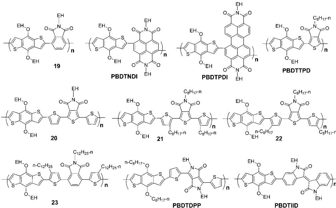
Scheme 7 Molecular structures of BDT-based polymers with amide, imide and diimide-containing conjugated components.
