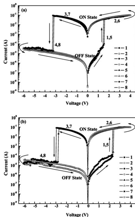
Fig. 5 Current–voltage ( I – V ) curves of (a) APTT-6FDA, and (b) 3SDA-6FDA. Reprinted with permission from ref. 12. Copyright 2009, American Chemical Society.
