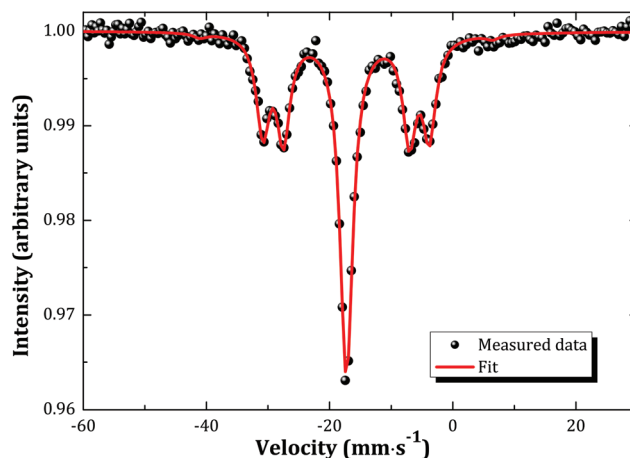
Fig. 5 Mössbauer spectrum of \alpha - \text{Na}_3\text{NbO}_4 recorded at 4.2 K and fitted to the model (see text).
