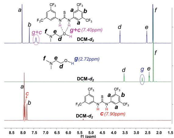
Fig. 5 ^1\text{H} NMR spectra of TU-S, DMEA and TU-S/DMEA (1:1) mixture (500 M, 25 °C, \text{CD}_2\text{Cl}_2 , for full spectra see Fig. S12†).
