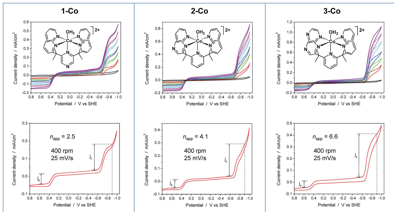
Fig. 6 RDEV of the series of cobalt catalysts. Panels: axial isomer 1-Co , [(ax-PY4PZMe 2 )Co(OH 2 ) 2 ] 2+ ; equatorial isomer 2-Co , [(eq-PY4PZMe 2 )Co(OH 2 ) 2 ] 2+ ; and catalyst 3-Co , [(PY3PZ2Me 2 )Co(OH 2 ) 2 ] 2+ . Top: rotation rates of 100–3600 rpm; bottom: apparent n_{app} based on 1e^- Co(III/II) couple at 400 rpm. Conditions: 0.3 mM catalyst, 0.1 M pH 7 KPBs, 0.1 M KNO 3 , 25 mV s -1 scan rate, glassy carbon electrode (3 mm dia).
