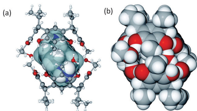
Fig. 2 Dimeric capsule, (TDAC) 2+ @1·H 2 O·MeOH 2 shown in (a) as ball and stick with the calculated cavity in transparent grey colour and the guest (TDAC) 2+ as CPK to illustrate the very tight encapsulation and (b) as the CPK model.
