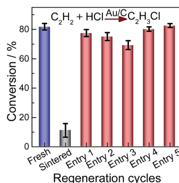
Fig. 7 Relative catalytic activity of acetylene hydrochlorination over the fresh, sintered and regenerated Au/C catalysts. Entries 1–3: sintered Au/C regenerated directly with \text{CHI}_3 at 40^\circ\text{C} ; Entries 4 and 5: sintered Au/C catalyst regenerated with \text{CHI}_3 containing \text{HAuCl}_4 (0.002 M) at 40^\circ\text{C} .
