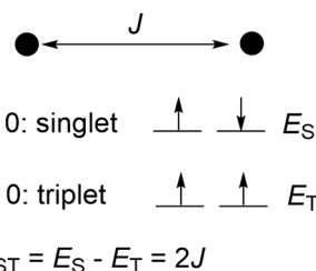
Scheme 1 The electron exchange integral, electronic configurations and singlet–triplet energy gap of a diradical.
