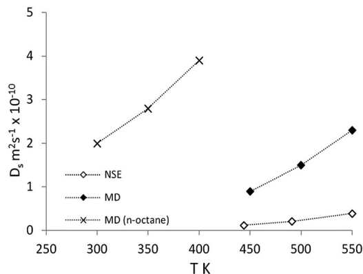
Fig. 9 Comparison of diffusion coefficients of isobutane from NSE ( \diamond ) and MD ( \blacksquare ) compared with previous simulations of n -octane diffusion in ref. 51 ( \times ). Reproduced from ref. 59 with permission from the American Chemical Society.
