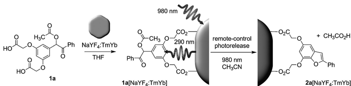
Fig. 5 UCNP-assisted photolysis at surfaces of UCNP. Decoration of UCNP with 3',5'-di(carboxymethoxy)benzoin cage 1a produces the remote-control release system ( 1a [NaYF 4 :TmYb]), which can be triggered by indirect irradiation with NIR light to generate 2a [NaYF 4 :TmYb] and release a carboxylic acid. Reproduced with permission. 71 Copyright 2010, Wiley-VCH Verlag GmbH & Co. KGaA.
