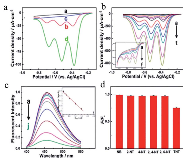
Fig. 10 (a) Differential pulse voltammograms (DPVs) recorded at a bare glassy carbon (GC) electrode (a, b) and a CDs/GC electrode (c, d) in 0.1 M \text{N}_2 -saturated PBS (containing 0.2 M KCl) at a pH of 7.0 with (b, d) and without (a, c) 5 \mu M TNT. (b) DPVs recorded corresponding to different concentrations of TNT at a CDs/GC electrode (inset: magnification of the low-concentration region) (a–t: blank, 1 nM, 5 nM, 10 nM, 20 nM, 30 nM, 80 nM, 130 nM, 230 nM, 330 nM, 830 nM, 1.33 \mu M, 2.33 \mu M, 3.33 \mu M, 4.33 \mu M, 9.33 \mu M, 14.33 \mu M, 19.33 \mu M, 29.33 \mu M, and 39.33 \mu M). (c) The PL intensity responding to different concentrations of TNT and the corresponding calibration plot (c–a–c–j: blank, 1 nM, 10 nM, 50 nM, 150 nM, 250 nM, 500 nM, 1 \mu M, 1.5 \mu M, and 2.5 \mu M). (d) PL changes corresponding to concentrations of 5 \mu M of different interfering substances, as well as 0.5 \mu M TNT. (Reprinted with permission from ref. 148. Copyright 2015, American Chemical Society.)
