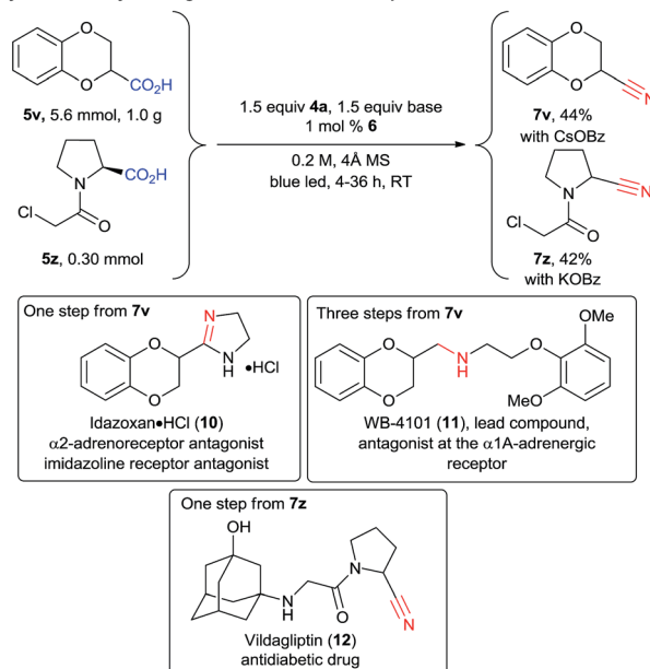
Scheme 5 Sun light experiment (A), scale up (B) and synthesis of key building blocks (C).
