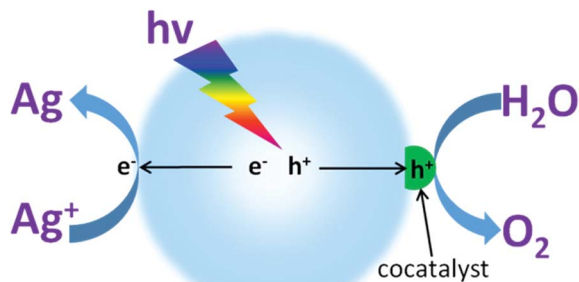
Fig. 10 Schematic illustration of photocatalytic water oxidation for \text{O}_2 evolution in the presence of an electron acceptor driven by a semiconductor modified with \text{O}_2 evolution cocatalysts.
