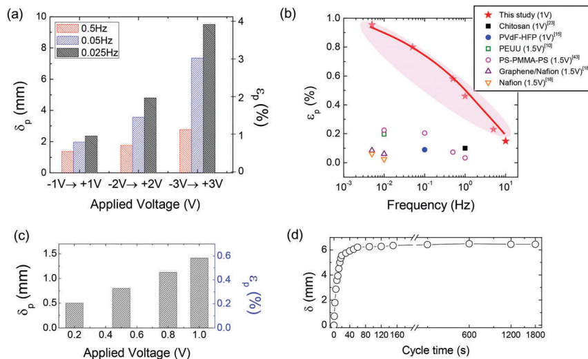
Fig. 7 (a) Displacement ( \delta )/bending strain ( \epsilon_p )–frequency–voltage dependency of the actuator comprising a sulfonated block copolymer and ionic liquid with \pm 3 V. (b) Strain–frequency–voltage dependency of the actuator, compared with those reported in literature with a focus on low-voltage operation. (c) Actuation performance obtained under sub-1 V conditions measured at the tip position of the actuator strip every 1 s with step changes in voltage from 0 to 0.2, 0 to 0.5 and 0 to 0.8 V. (d) Time-dependent displacement of the actuator at 3 V, demonstrating the absence of back relaxation. Figure is adapted from ref. 73 with the permission of the Nature publishing group.
